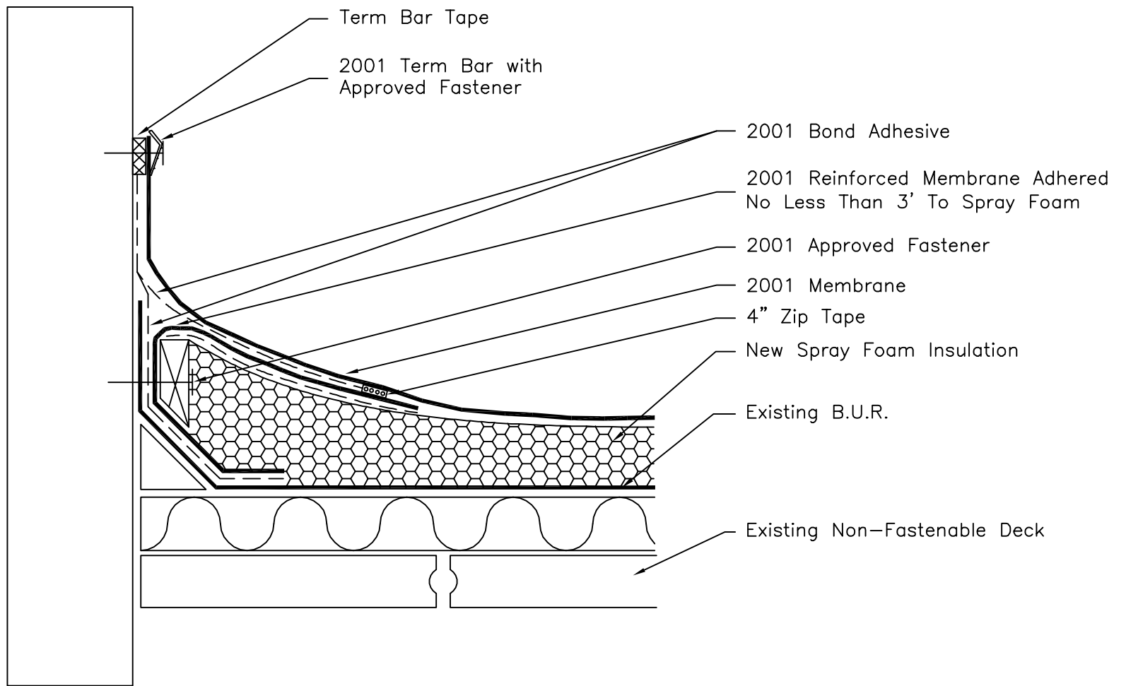
2001 Co. Spray Foam Over Existing Built Up Roof. Air Sealed with Reinforced Membrane Adhered To Existing Flushing and Fliped Back For A Shear Skirt Attachment Of The Field Membrane.
