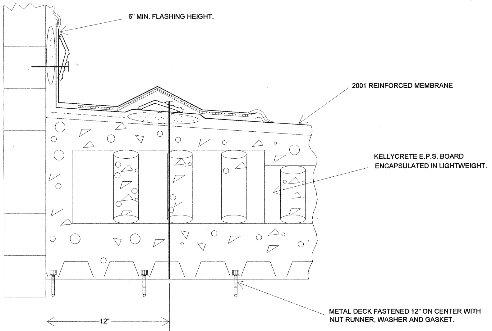
AIR SEAL ROOF MEMBRANE; 2001 REINFORCED MEMBRANE DIRECT TO LIGHTWEIGHT DECK; 12" FROM EDGE.
