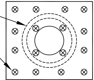
FASTENING PATTERN
